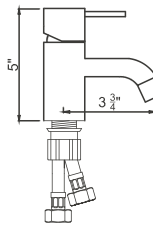
SINGLE LEVER BASIN MIXER FLORENTINE
