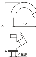
SWAN NECK REG. SPOUT MARC, DELTA, CROWN, PRIZAM
