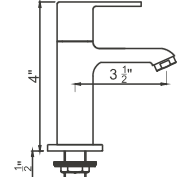
PRIZAM PILLAR COCK
