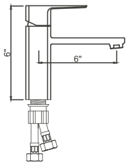
SINGLE LEVER BASIN MIXER TYCOON, ROLEX
