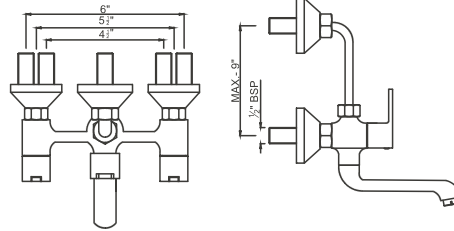
WALL MIXER 2 IN 1 CROWN, PRIZAM WALL MIXER 3 IN 1 CROWN, PRIZAM
