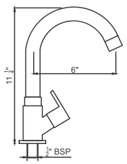
SWAN NECK PILLAR WITH EXT. SPOUT TYCOON, ROLEX
