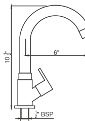
SWAN NECK PILLAR WITH EXT. SPOUT MARC, DELTA, CROWN, PRIZAM
